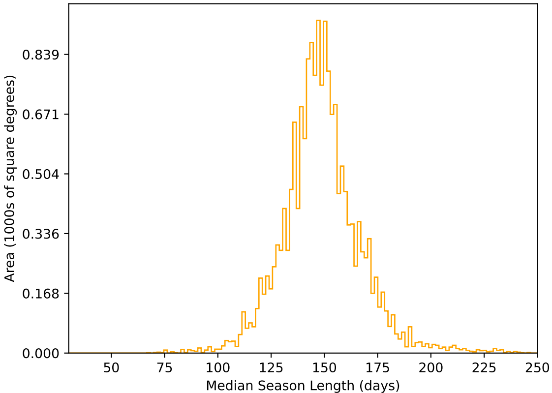
baseline_v3.2_10yrs WFD r band: Median Season Length
