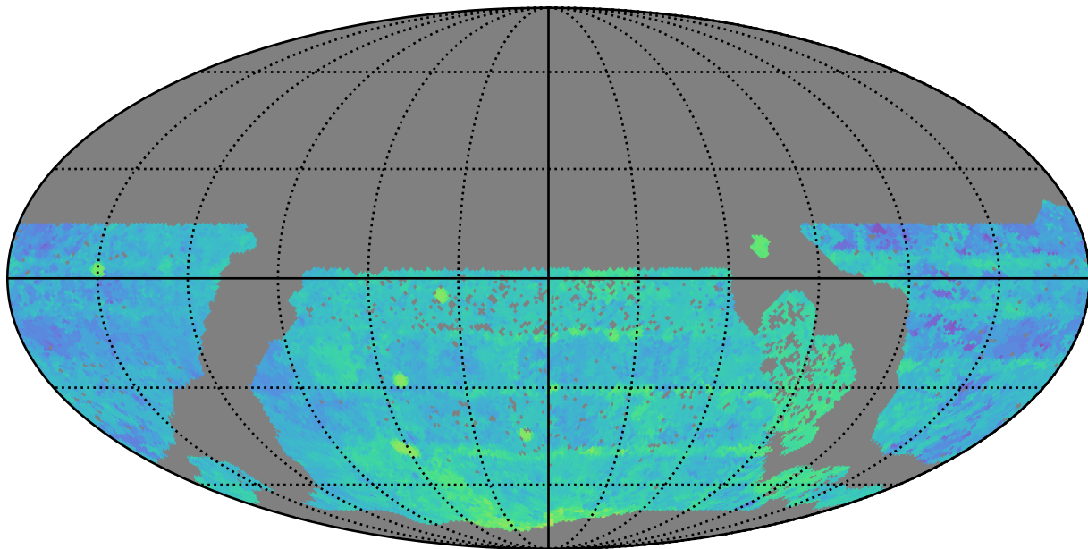
baseline_v3.2_10yrs WFD i band: Median Season Length
