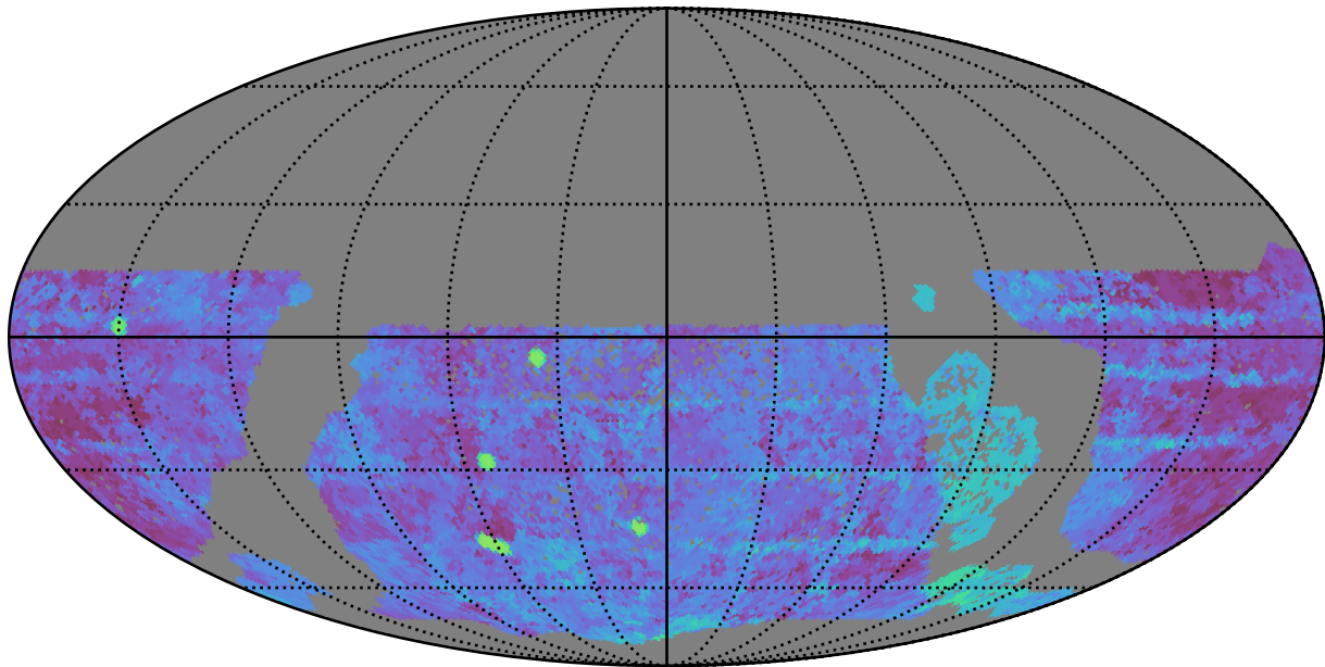
baseline_v3.2_10yrs WFD g band: Median Season Length
