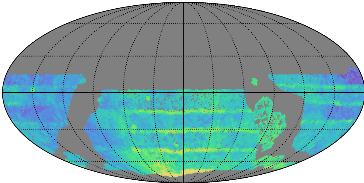
baseline_v3.2_10yrs WFD all bands: Median Season Length
