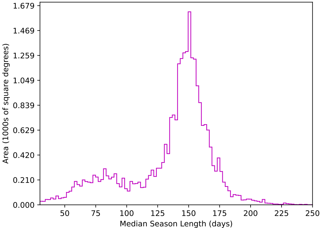
baseline_v3.2_10yrs All sky z band: Median Season Length
