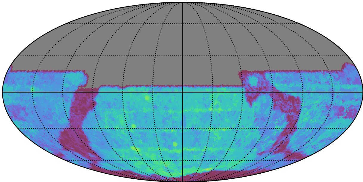
baseline_v3.2_10yrs All sky y band: Median Season Length
