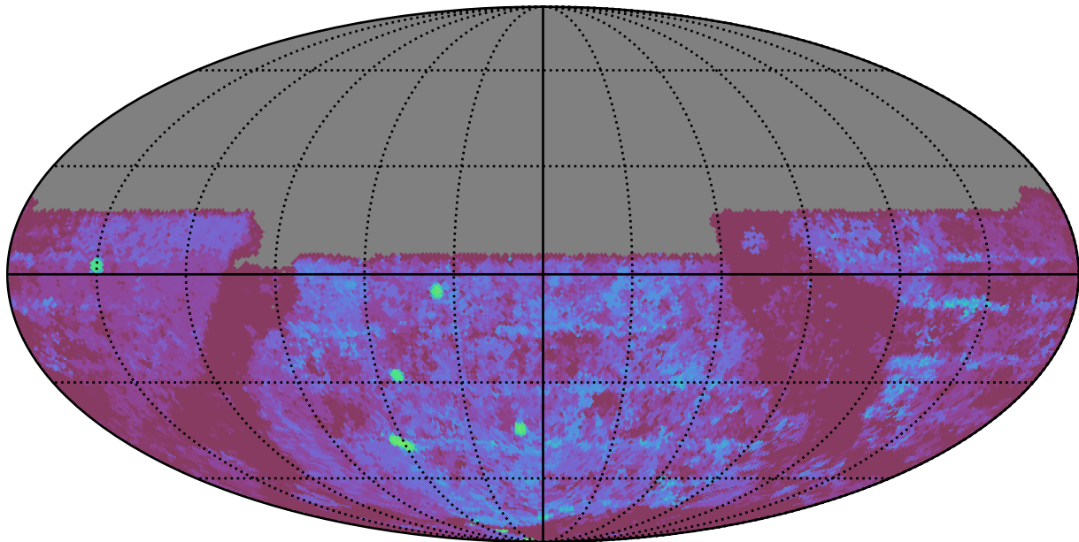
baseline_v3.2_10yrs All sky u band: Median Season Length
