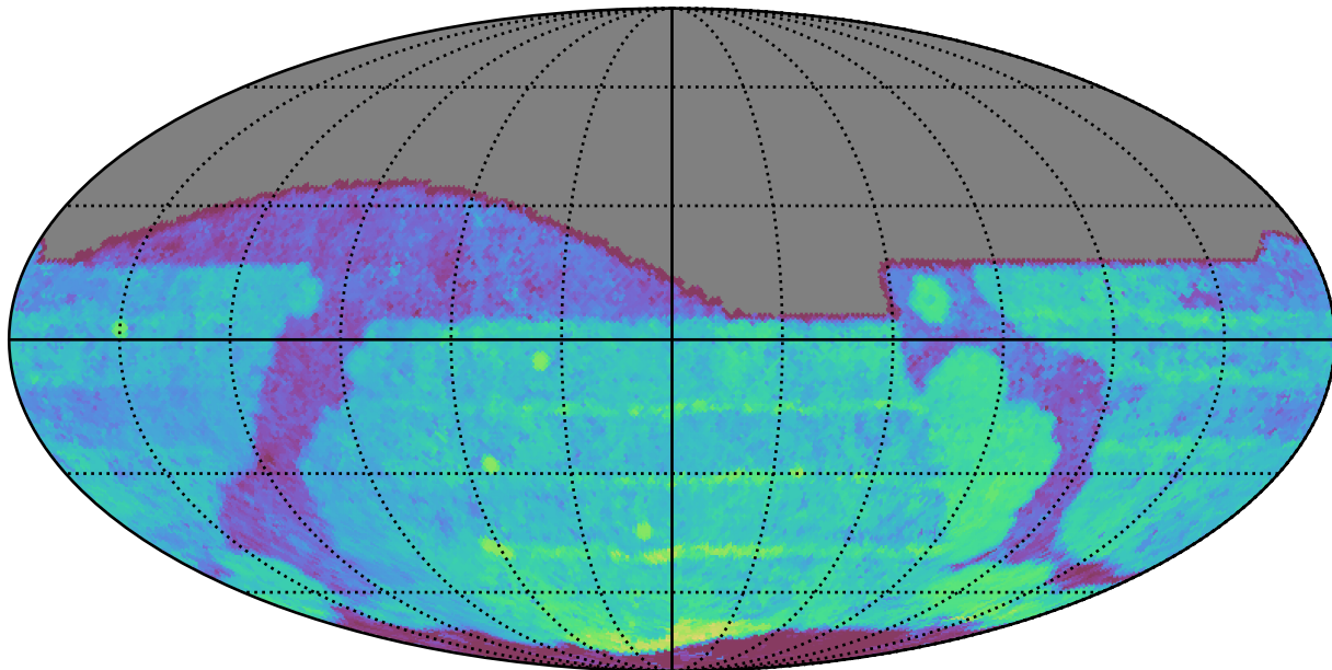
baseline_v3.2_10yrs All sky r band: Median Season Length
