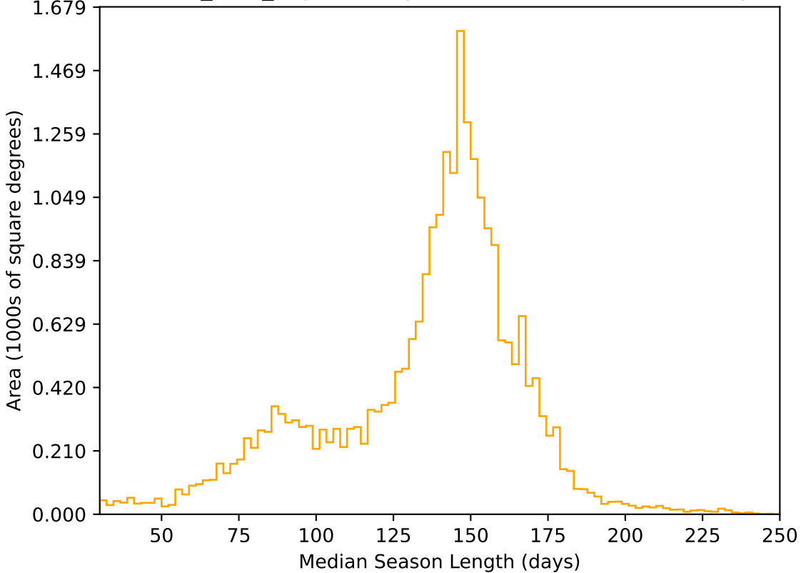
baseline_v3.2_10yrs All sky r band: Median Season Length
