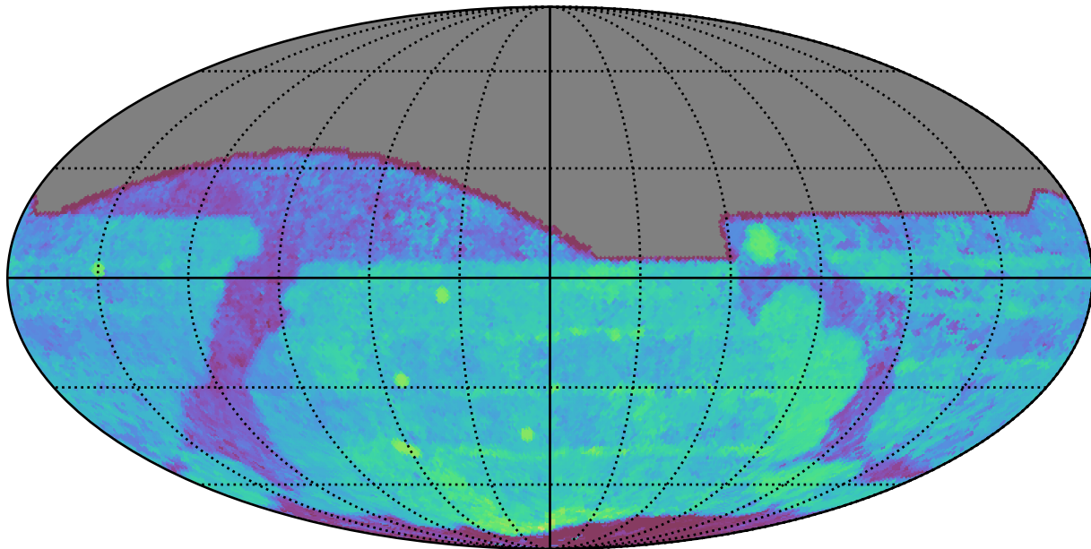
baseline_v3.2_10yrs All sky i band: Median Season Length
