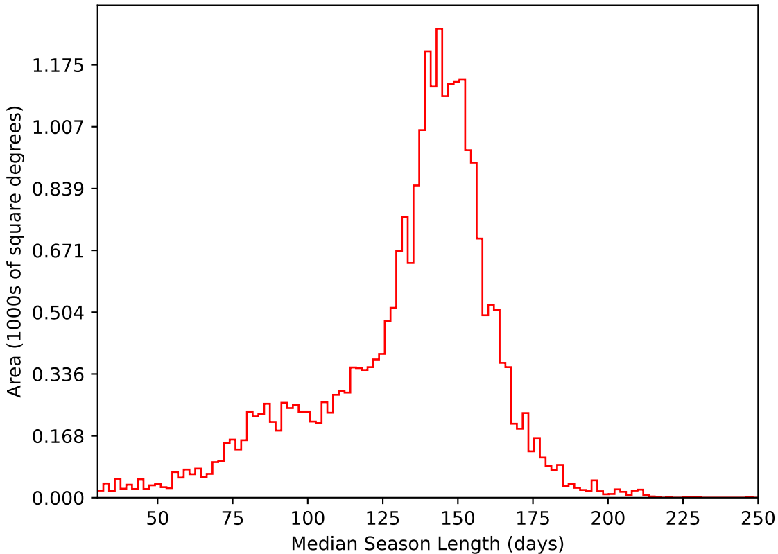
baseline_v3.2_10yrs All sky i band: Median Season Length
