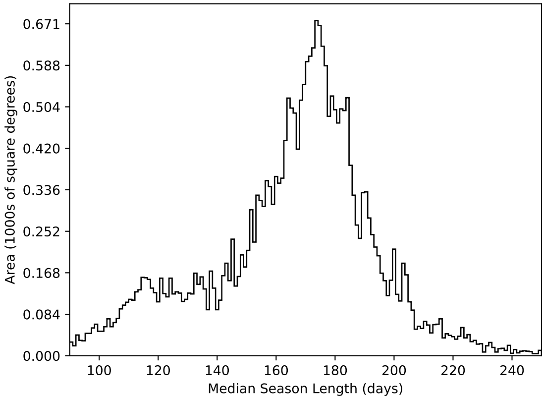
baseline_v3.2_10yrs All sky all bands: Median Season Length
