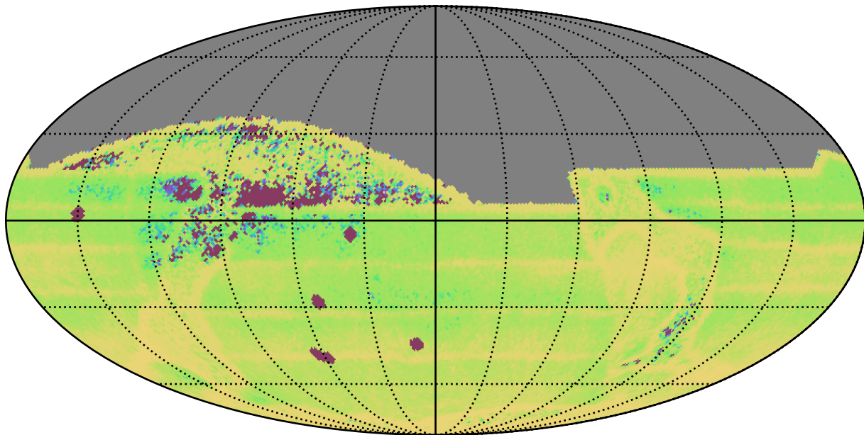
baseline_v3.2_10yrs All sky: Median Intra-Night Gap
