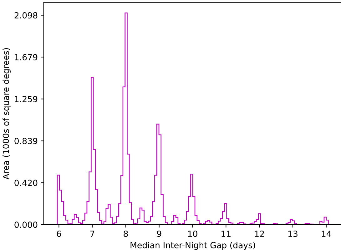
baseline_v3.2_10yrs WFD z band: Median Inter-Night Gap
