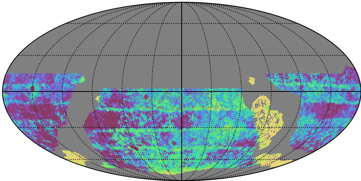
baseline_v3.2_10yrs WFD y band: Median Inter-Night Gap
