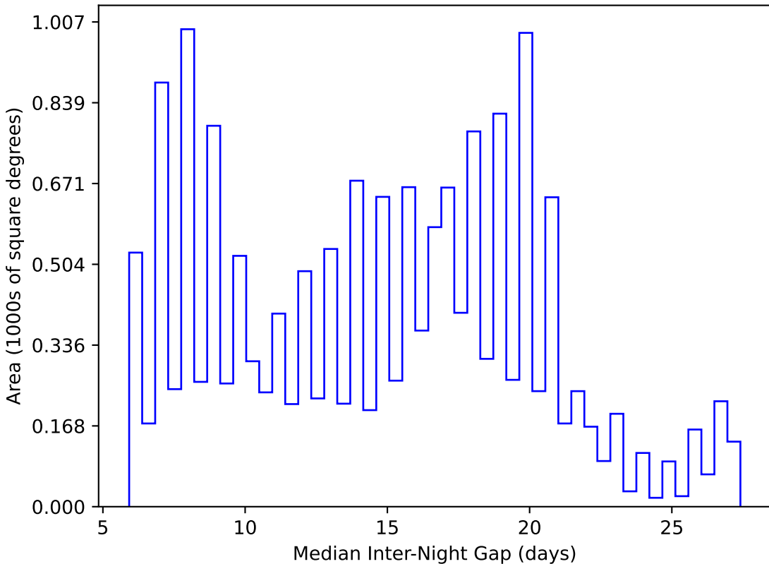
baseline_v3.2_10yrs WFD y band: Median Inter-Night Gap
