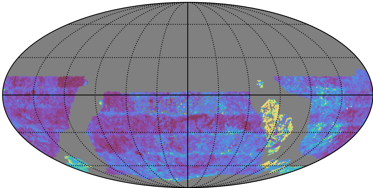
baseline_v3.2_10yrs WFD u band: Median Inter-Night Gap
