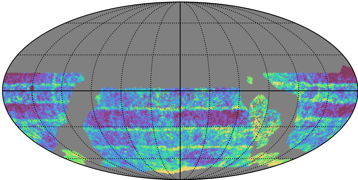
baseline_v3.2_10yrs WFD r band: Median Inter-Night Gap
