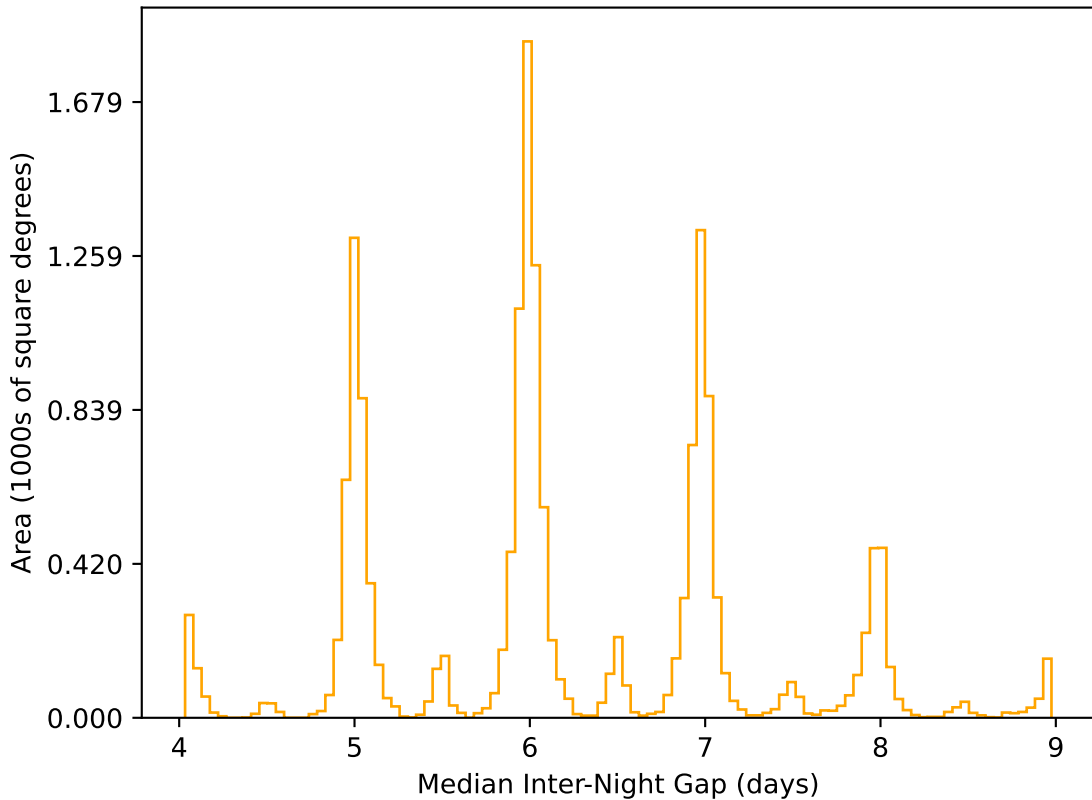
baseline_v3.2_10yrs WFD r band: Median Inter-Night Gap
