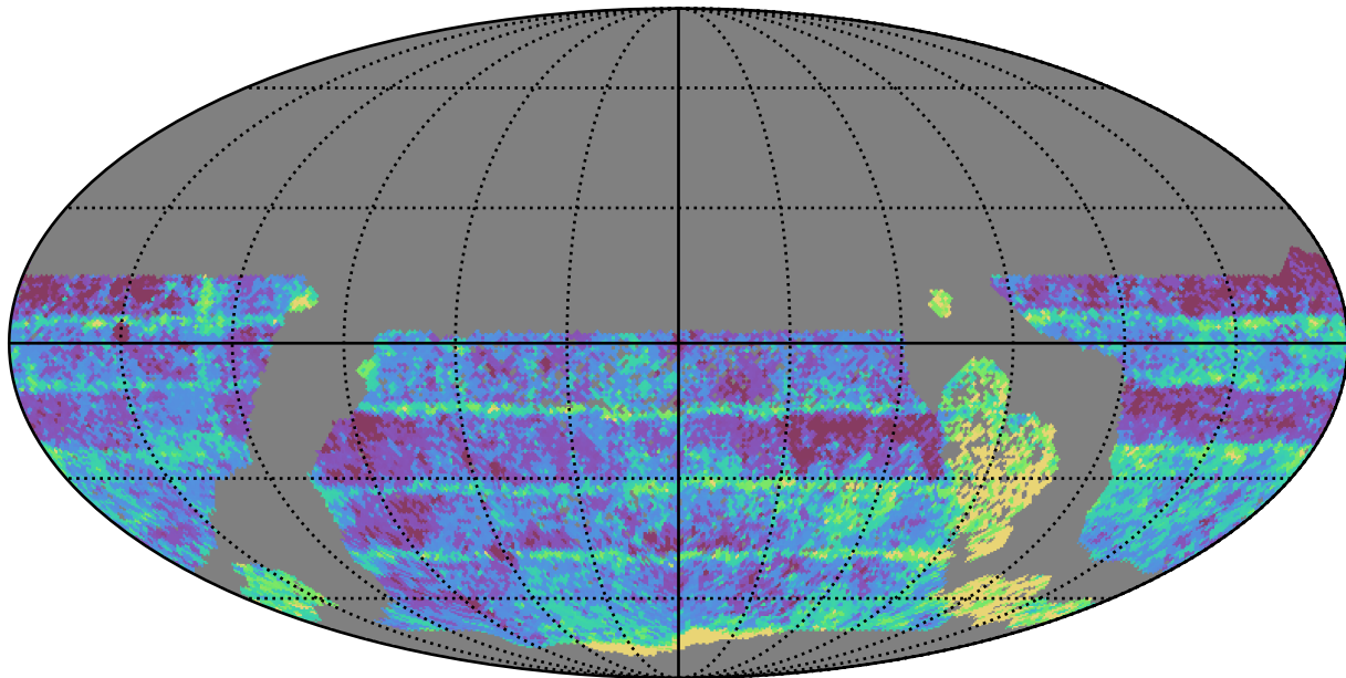
baseline_v3.2_10yrs WFD i band: Median Inter-Night Gap
