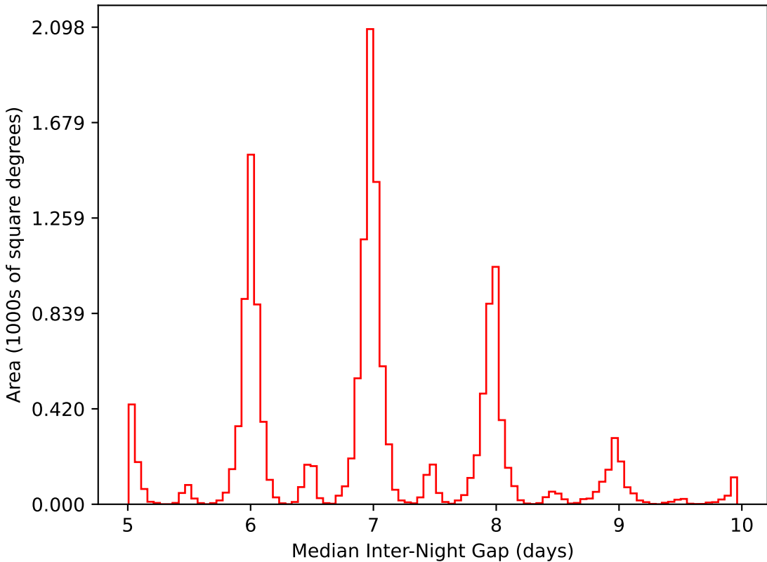
baseline_v3.2_10yrs WFD i band: Median Inter-Night Gap
