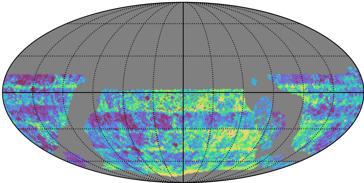
baseline_v3.2_10yrs WFD g band: Median Inter-Night Gap
