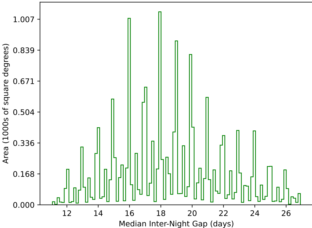
baseline_v3.2_10yrs WFD g band: Median Inter-Night Gap
