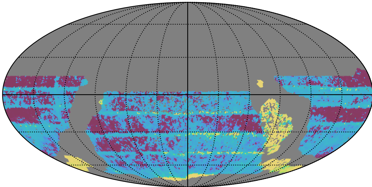
baseline_v3.2_10yrs WFD all bands: Median Inter-Night Gap
