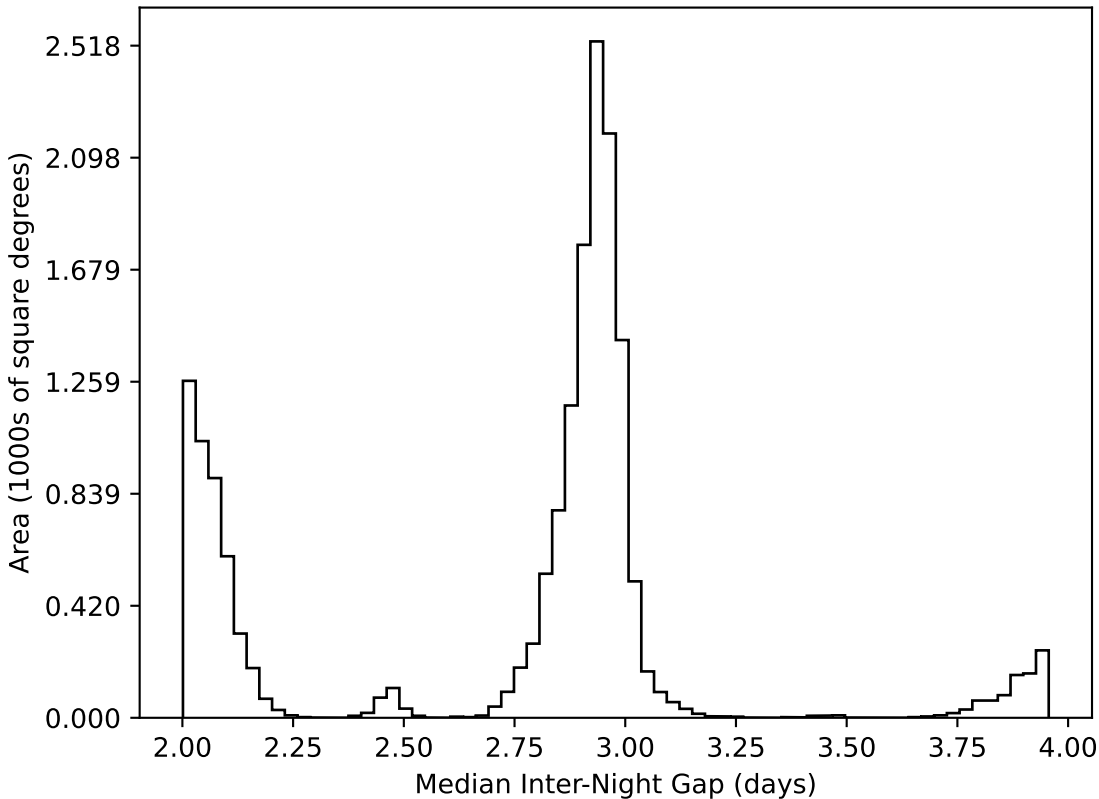
baseline_v3.2_10yrs WFD all bands: Median Inter-Night Gap
