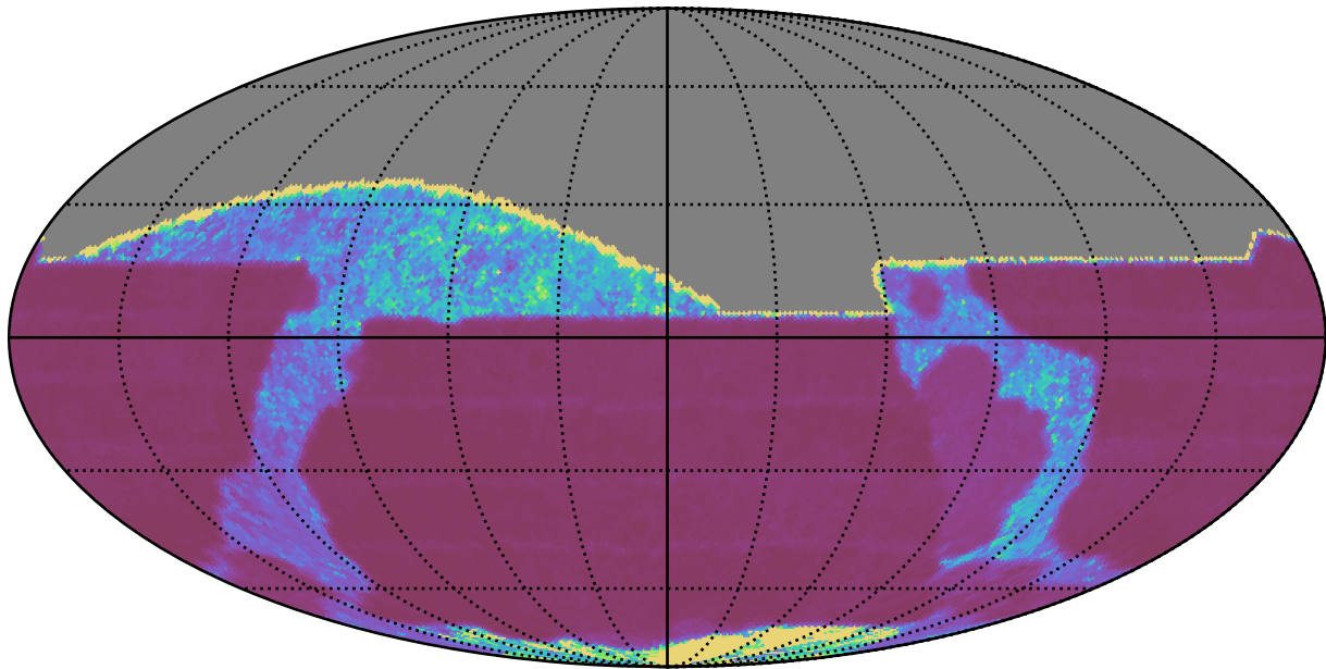
baseline_v3.2_10yrs All sky z band: Median Inter-Night Gap
