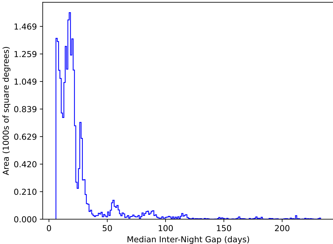
baseline_v3.2_10yrs All sky y band: Median Inter-Night Gap
