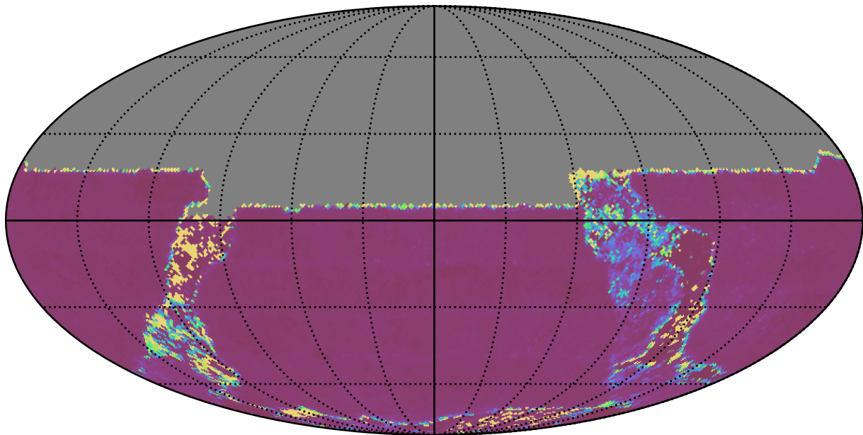
baseline_v3.2_10yrs All sky u band: Median Inter-Night Gap
