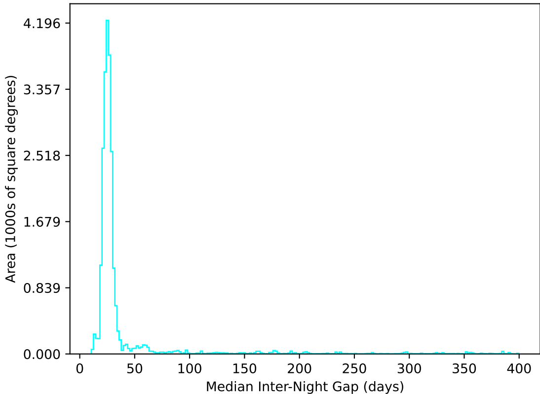
baseline_v3.2_10yrs All sky u band: Median Inter-Night Gap
