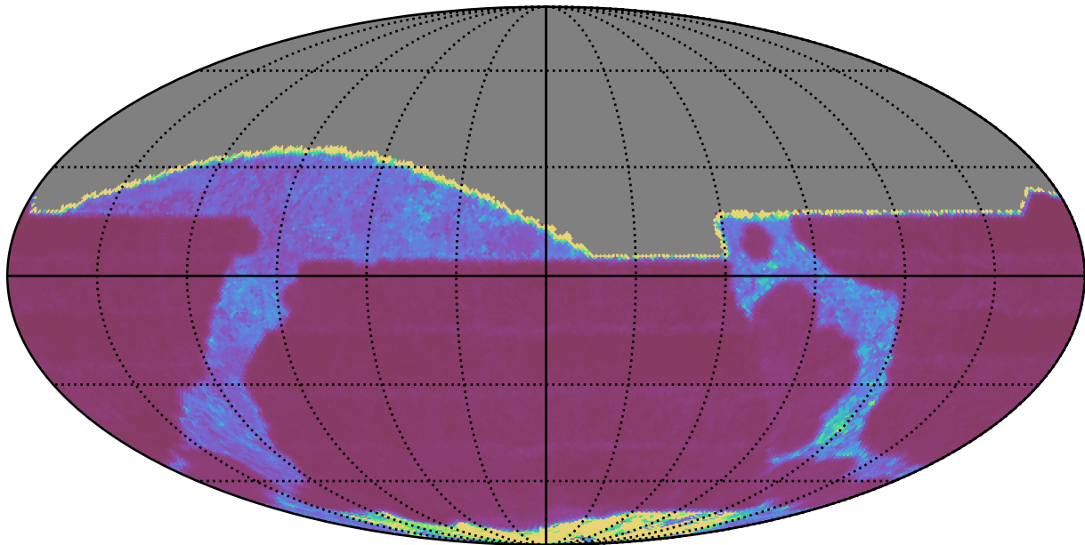
baseline_v3.2_10yrs All sky r band: Median Inter-Night Gap
