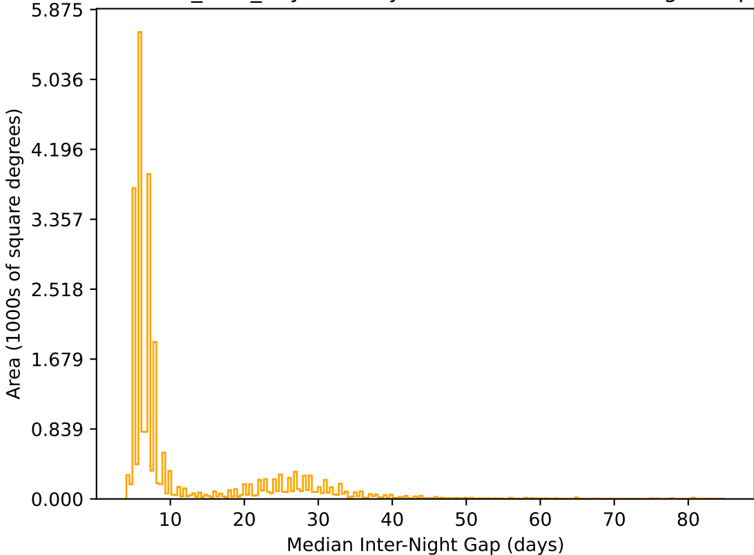
baseline_v3.2_10yrs All sky r band: Median Inter-Night Gap
