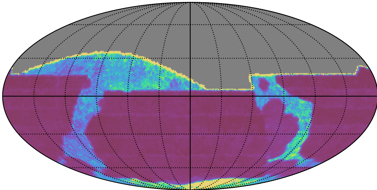
baseline_v3.2_10yrs All sky i band: Median Inter-Night Gap
