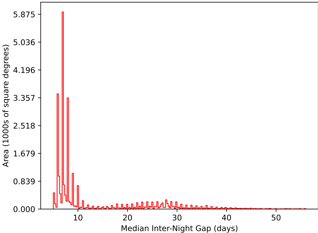
baseline_v3.2_10yrs All sky i band: Median Inter-Night Gap
