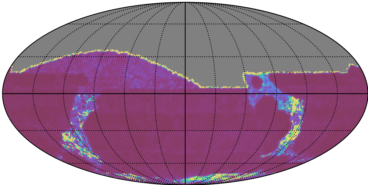
baseline_v3.2_10yrs All sky g band: Median Inter-Night Gap
