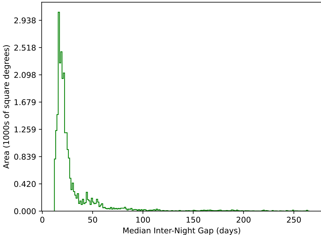
baseline_v3.2_10yrs All sky g band: Median Inter-Night Gap
