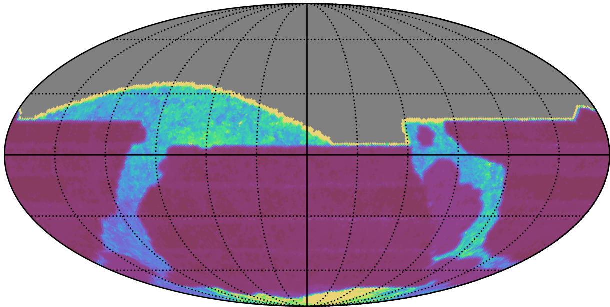
baseline_v3.2_10yrs All sky all bands: Median Inter-Night Gap
