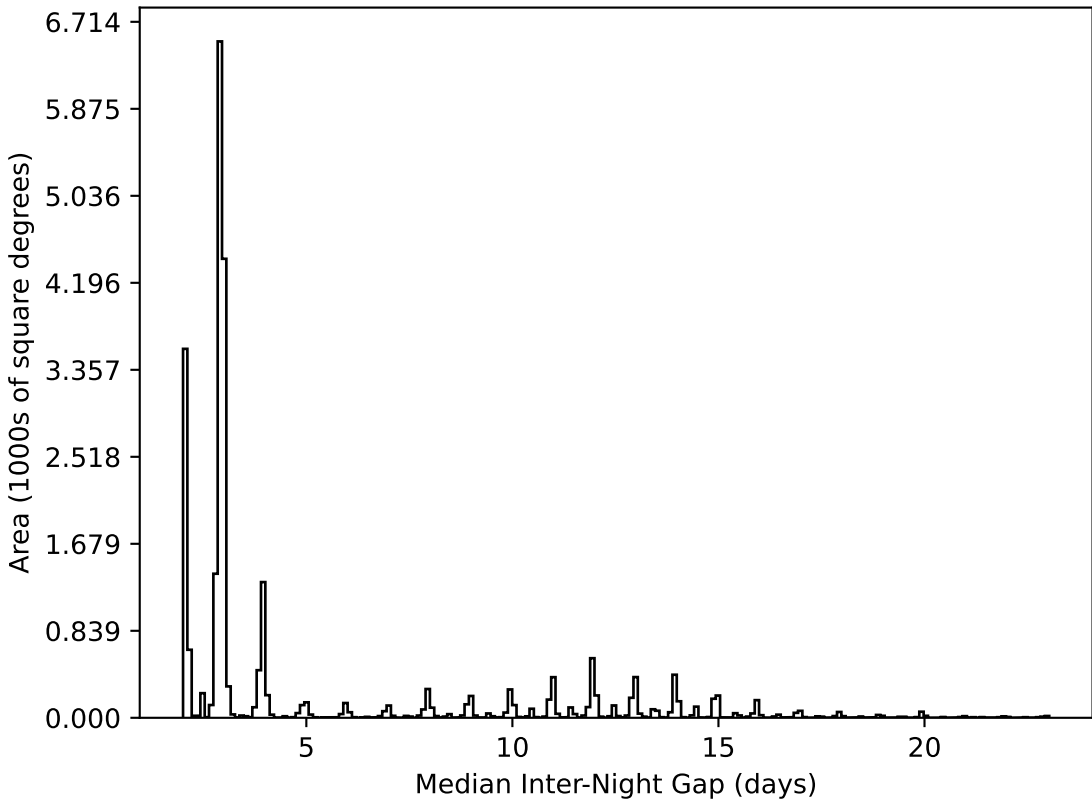
baseline_v3.2_10yrs All sky all bands: Median Inter-Night Gap
