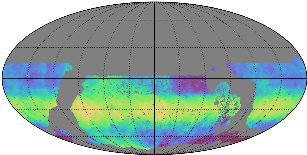
baseline_v3.2_10yrs WFD z band: Median HA
