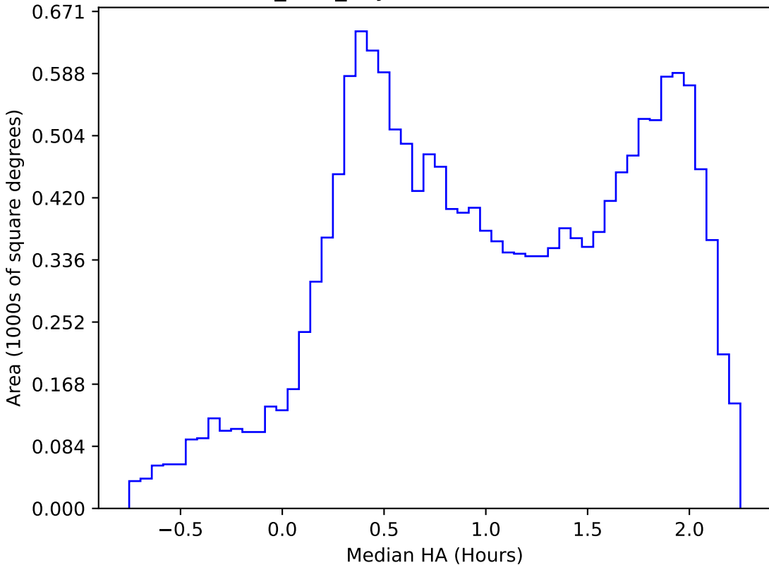
baseline_v3.2_10yrs WFD z band: Median HA
