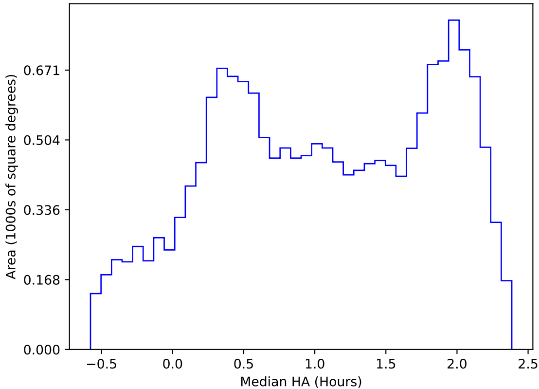
baseline_v3.2_10yrs WFD y band: Median HA
