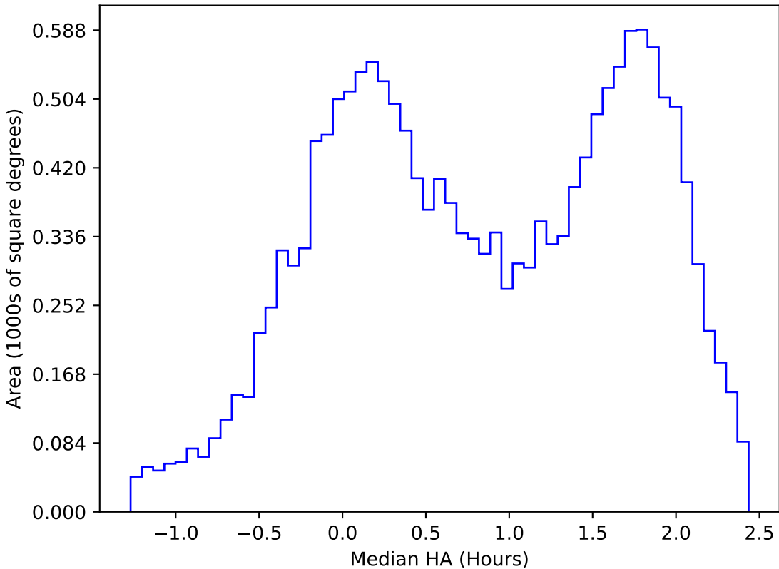
baseline_v3.2_10yrs WFD u band: Median HA
