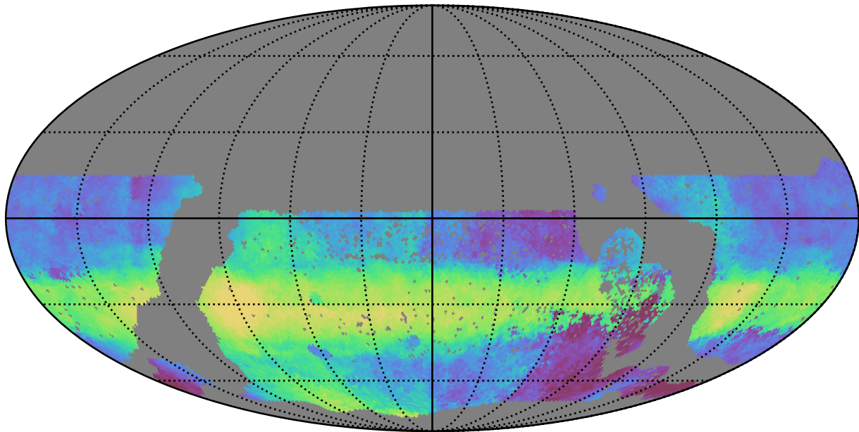
baseline_v3.2_10yrs WFD r band: Median HA
