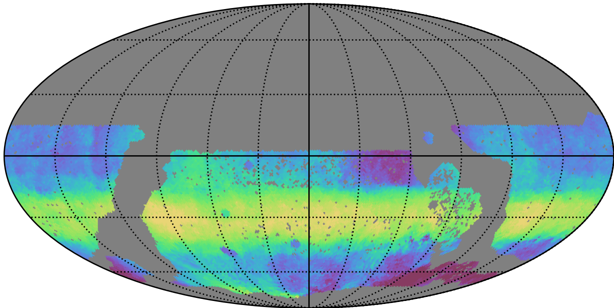
baseline_v3.2_10yrs WFD i band: Median HA
