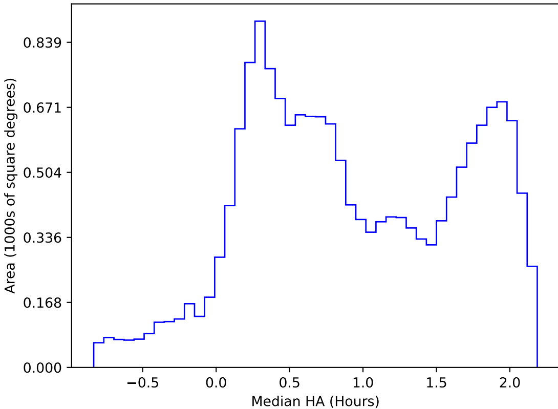
baseline_v3.2_10yrs WFD i band: Median HA
