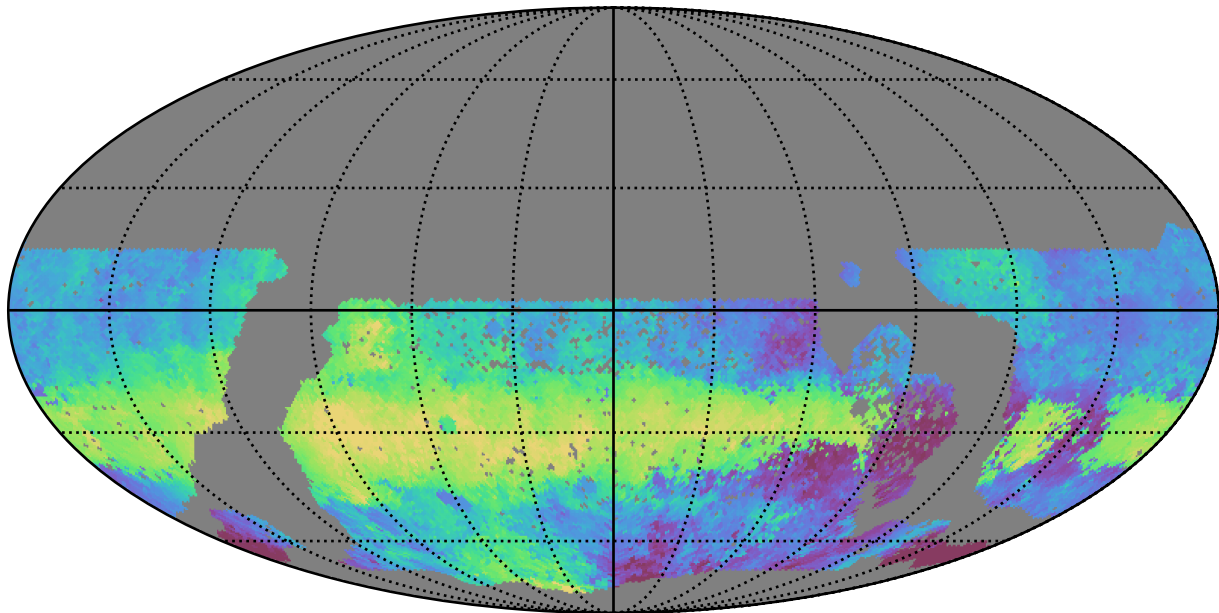
baseline_v3.2_10yrs WFD g band: Median HA
