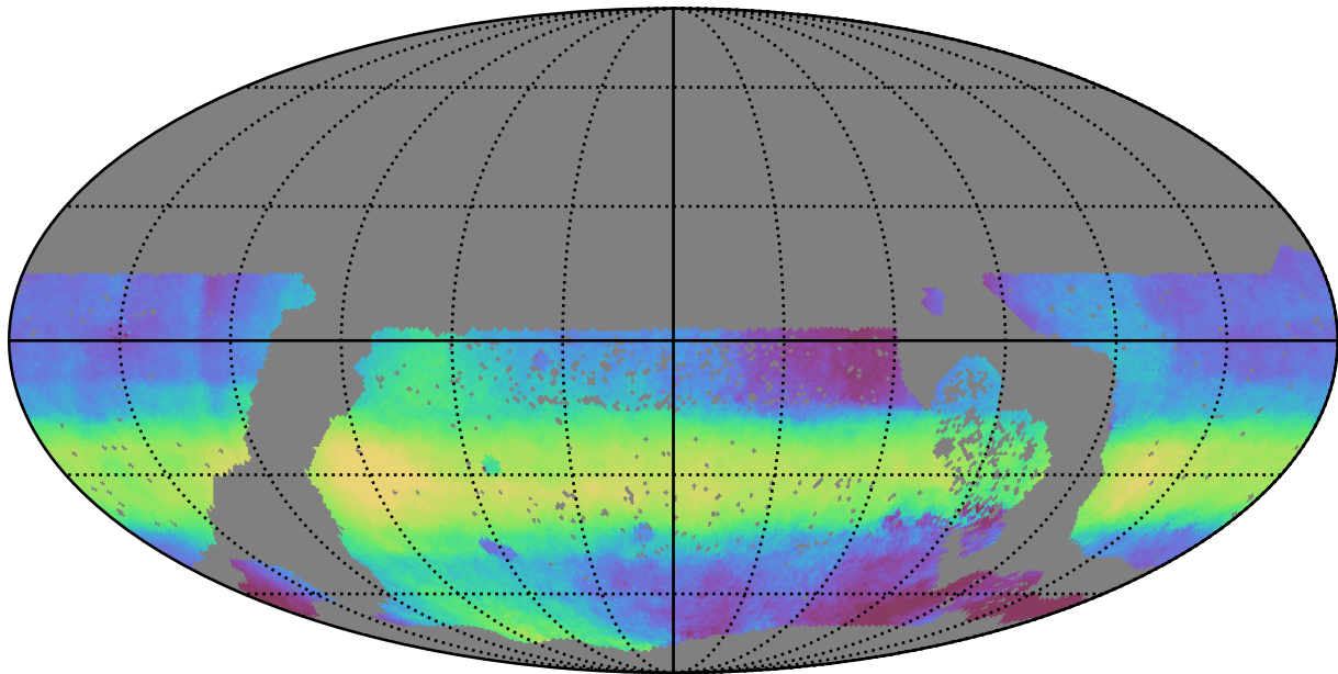
baseline_v3.2_10yrs WFD all bands: Median HA
