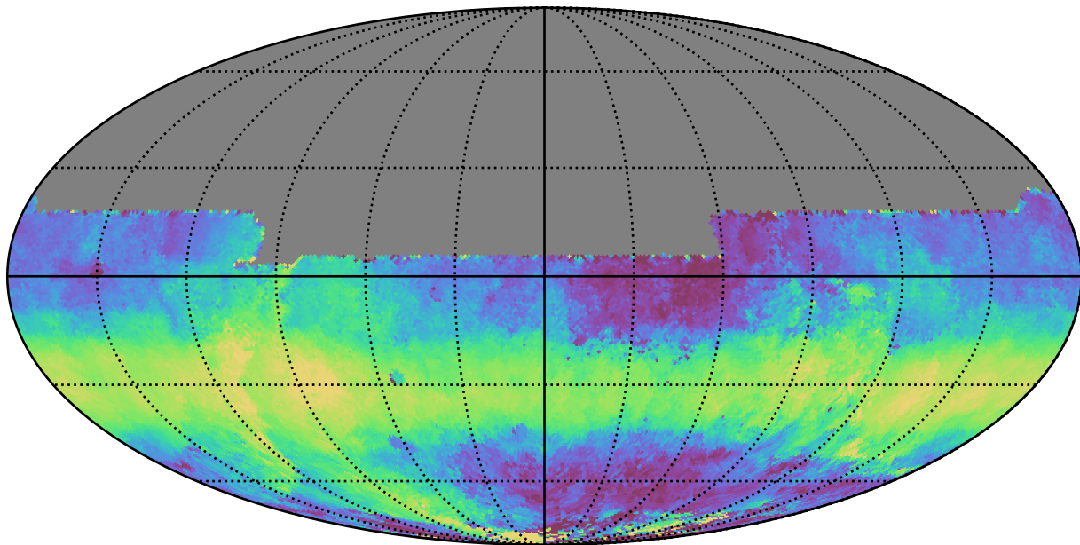
baseline_v3.2_10yrs All sky y band: Median HA
