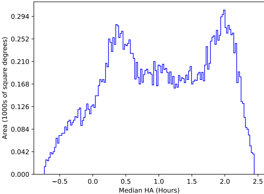
baseline_v3.2_10yrs All sky y band: Median HA
