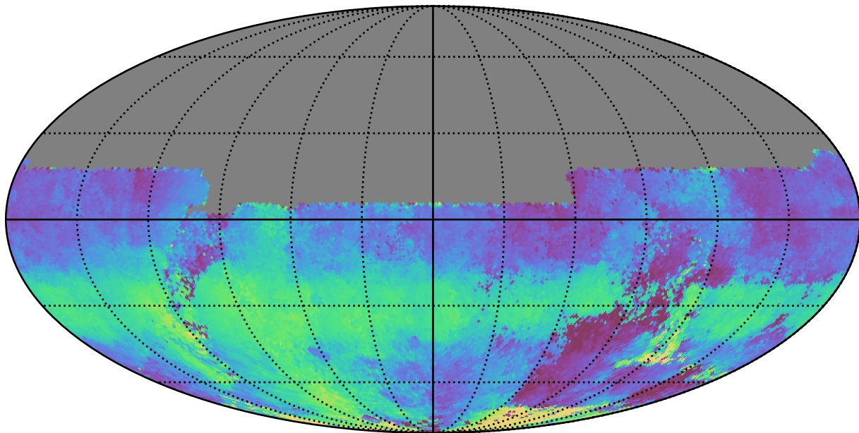
baseline_v3.2_10yrs All sky u band: Median HA
