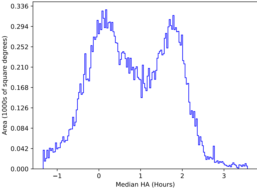
baseline_v3.2_10yrs All sky u band: Median HA
